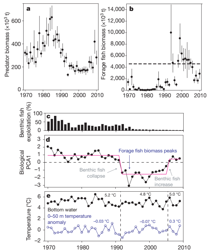
Figure 1 | Variability of the eastern Scotian Shelf ecosystem. a–e, Data (Supplementary Fig. 1) based on large-bodied benthic fish (a), their prey (forage fishes, b) with estimated carrying capacity (dashed line), benthic fish exploitation history expressed as annual per cent biomass removal (c), changing ecosystem structure based on the leading mode (PCA1) of biotic data spanning four trophic levels and the demarcation of regimes 29 of 22, 14 and 4 years duration (pink solid line) (d), and temperatures with averages shown for the three regimes (dashed vertical lines) (e). Vertical bars in a and b show \pm s.e.m. ( n = 27 ).
